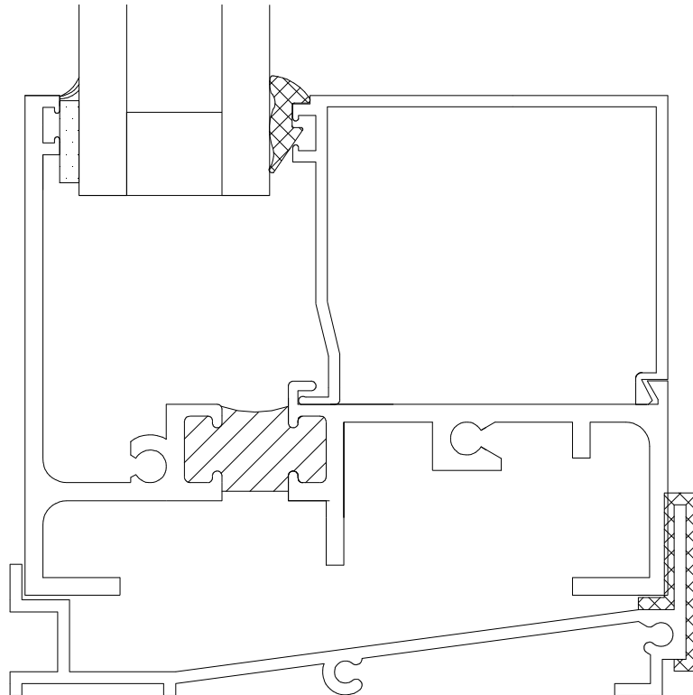
6 SILL @ FIXED
