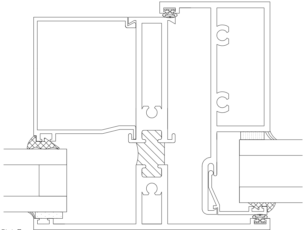
VERTICAL VENT @ RIGHT OF FIXED
