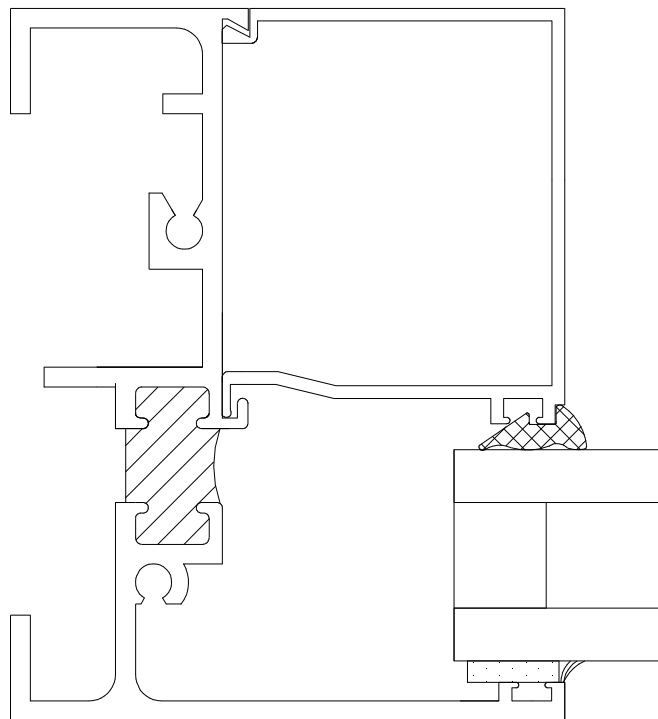
4 JAMB @ FIXED
