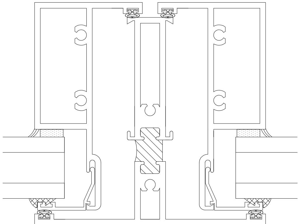
VERTICAL @ DOUBLE VENT
