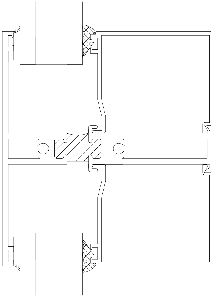
① 11 TYPICAL MULLION
