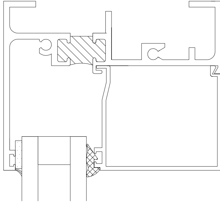
5 HEAD @ FIXED
